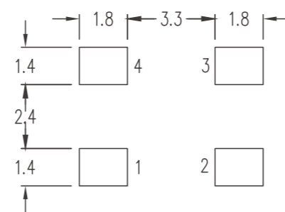
SOLDERING PATTERN (mm)
