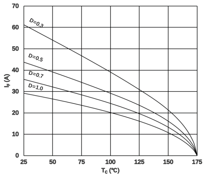
Figure 8. Forward Current as a Function of Temp
