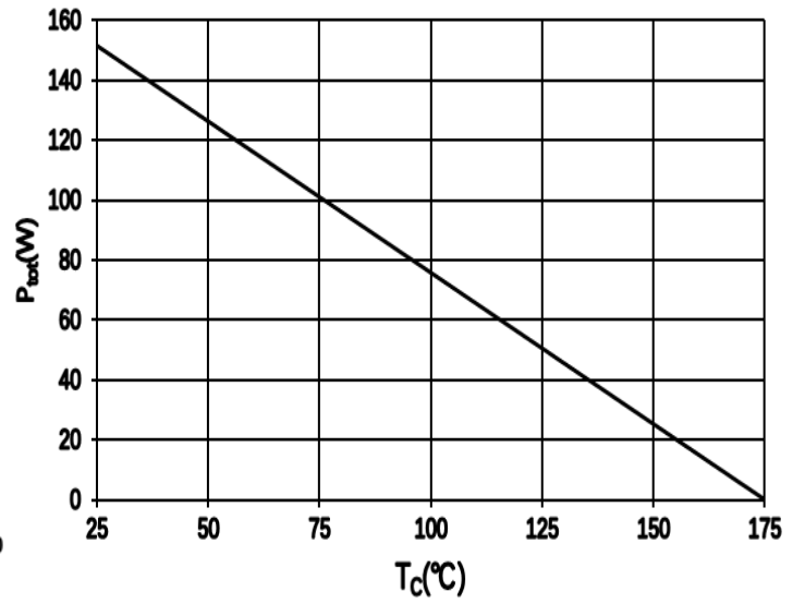
Figure 6. Power Derating
