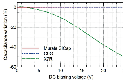
Fig.2: Capacitance variation vs DC biasing voltage @ BV 30 (for UBSC and MLCC technologies)
