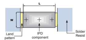
(0402 PCB footprint)
