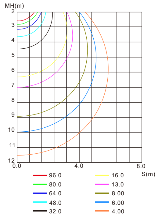
Spacing iso-illuminance curve
