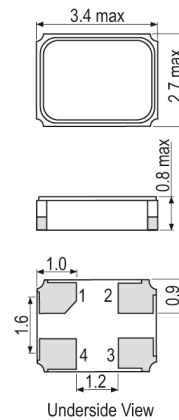
Underside View
