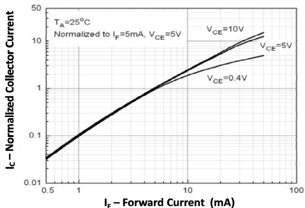
Fig 3 Normalized Collector Current vs Forward Current
