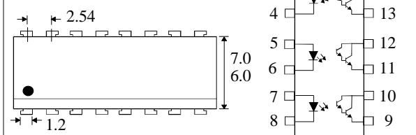
PS2502-4X PS2502-4
