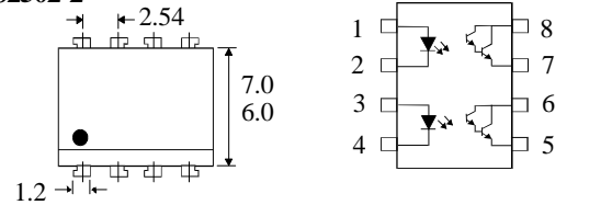
PS2502-2X PS2502-2
