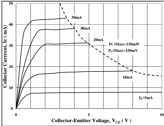
Fig 7 Collector Current vs Collector-Emitter Voltage
