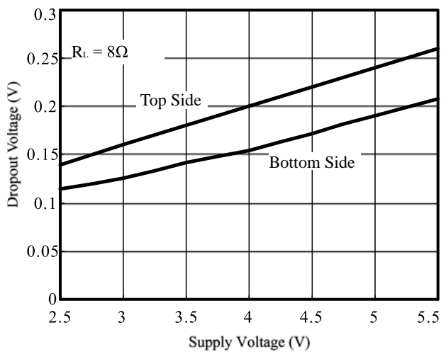
Figure 16 Dropout Voltage vs. Supply Voltage
