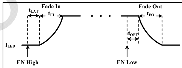
Figure 6 FIFO Function
