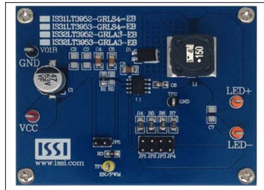
Figure 1: Photo of IS31LT3952_IS32LT3952 Evaluation Board
