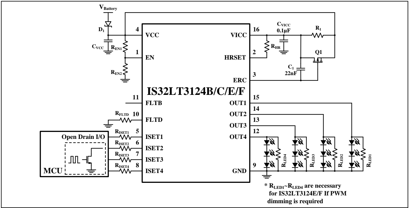
Figure 5 Typical Application Circuit With Open Drain I/O driving R_{ISET} Individual PWM Dimming (IS32LT3124B/C/E/F only) When PWM Generator is Close to Device
