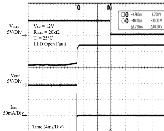
Figure 33 t_{FLT D}
