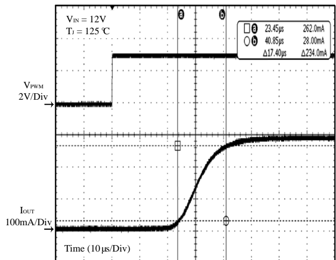
Figure 26 PWM On
