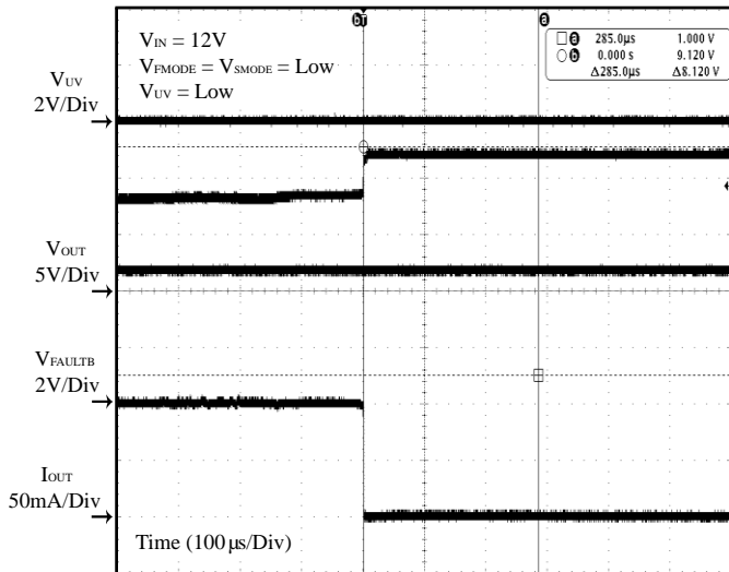
Figure 29 Output Open
