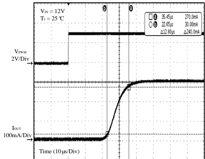
Figure 24 PWM On
