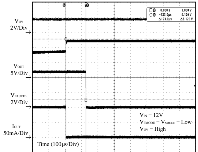
Figure 30 Output Open
