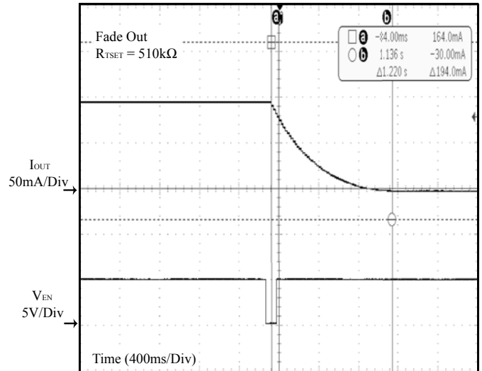
Figure 17 V_{EN} VS. I_{OUT}
