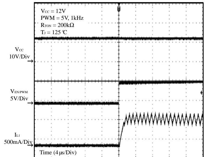
Figure 29 PWM On
