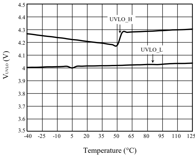
Figure 12 V_{UVLO} vs. Temperature
