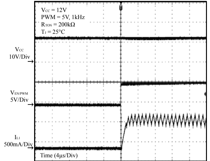
Figure 24 PWM On
