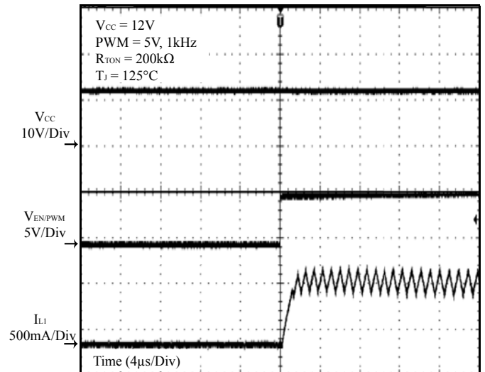
Figure 26 PWM On
