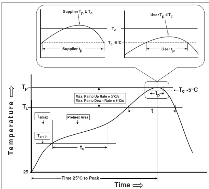
Figure 37 Classification Profile
