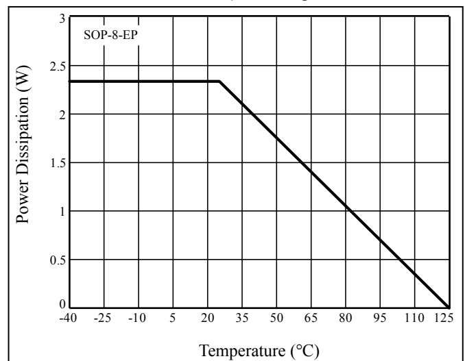
Figure 35 Dissipation Curve
