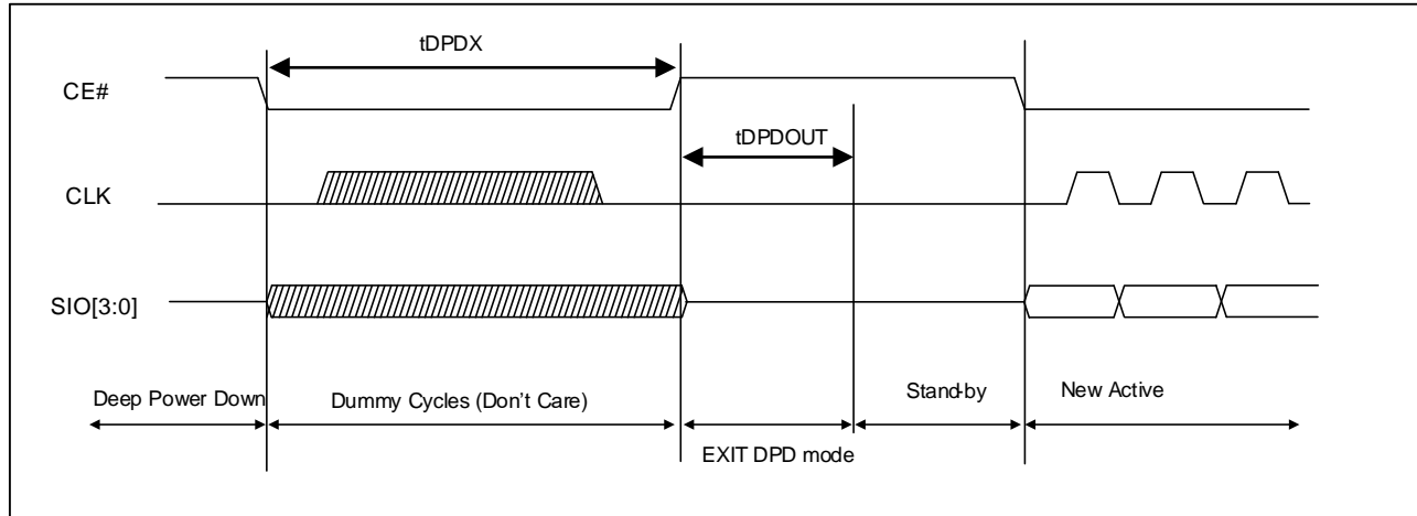
Figure 5.18 DEEP POWER DOWN EXIT Timing
