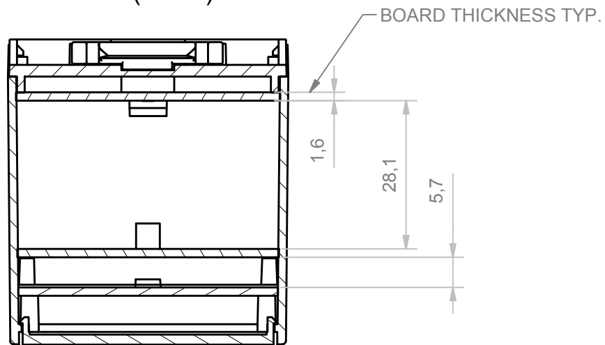
B-B (1:1)
