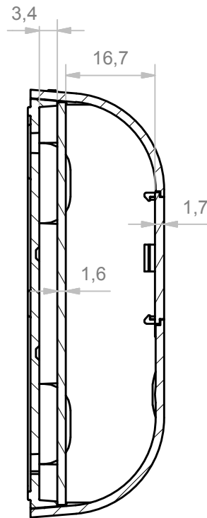
B-B (1:1)
