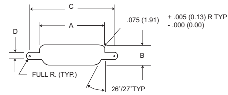
Figure 2 Rear Mounting
