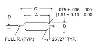
Figure 3 Rear Mounting
