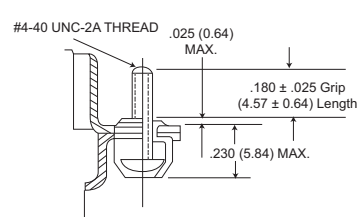
Low Profile (F173) Jackscrew (factory installed)
