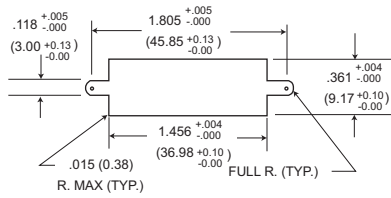
Figure 1 Front Mounting
