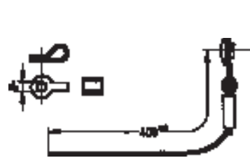
VG95234 Style KC with cord
