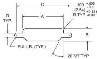
Figure 2 Rear Mounting
