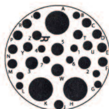
25-20 - 25-20* 3 #8 Twinax, 13 #16, 4 #12 Coax, 10 #20 N / Coax / Twinax I
