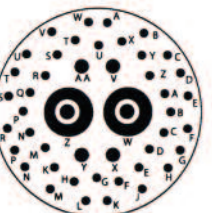
25-46 - 25-46 40 #20, 4 #16, 2 #8 Twinax
