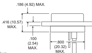
Plug
