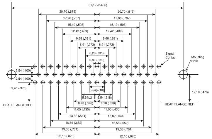
50 Contacts
