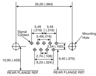
9 Contacts
