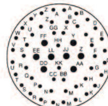
25-4 24-4† 25-4 48 #20, 8 #16 I
