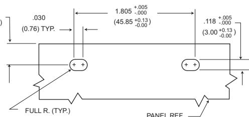
Figure 3 Edgeboard Mounting
