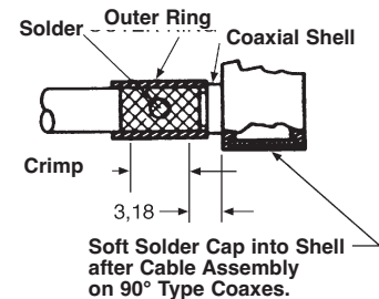
90° Coaxial
