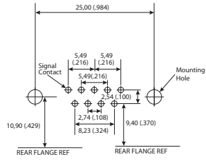
9 Contacts
