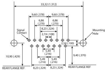
15 Contacts
