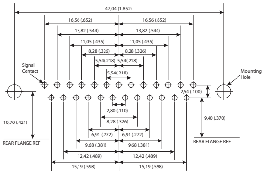
25 Contacts
