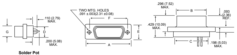
Solder Pot
