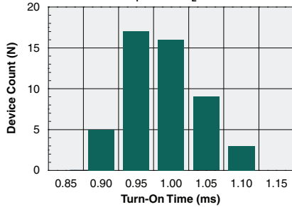
Typical Turn-On Time (N=50, I_F=5\text{mA} , I_L=100\text{mA} )
