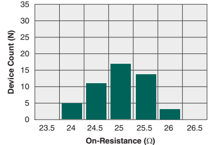
Typical On-Resistance Distribution (N=50, I_L=120\text{mA} , T_A=25^\circ\text{C} )
