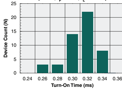
Typical Turn-On Time (N=50, I F =5mA, I L =60mA)
