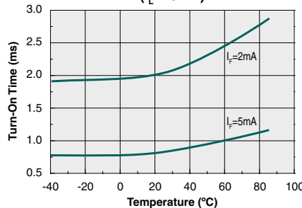
Typical Turn-On vs. Temperature ( I_L=70\text{mA} )
