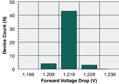
LED Forward Voltage Drop Distribution (N=50, I_F=5mA )
