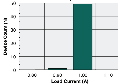
Typical Current Limit Distribution (N=50, I_F=5mA )
