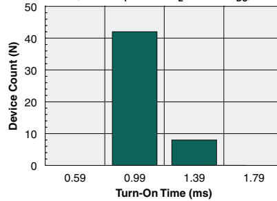
Typical Turn-On Time Distribution (N=50, I_F=5mA , I_L=100mA_{DC} )
