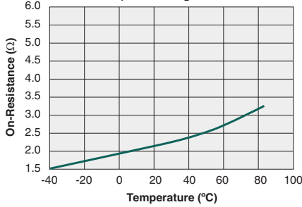
Typical On-Resistance vs. Temperature ( I_F=20\text{mA} , I_L=0.5\text{A} )
