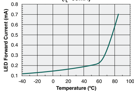
Typical LED Forward Current to Activate ( I_L=60\text{mA} )
