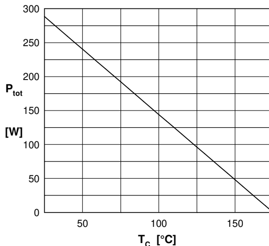
Fig. 4 Power derating
