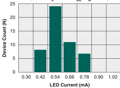
Typical I F for Switch Operation (N=50, I L =120mA DC , T A =25°C)
