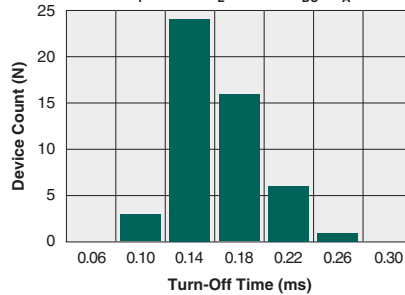
Typical Turn-Off Time (N=50, I F =2mA, I L =120mA DC , T A =25°C)
