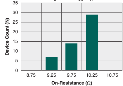
Typical On-Resistance Distribution (N=50, I L =120mA DC , T A =25°C)
