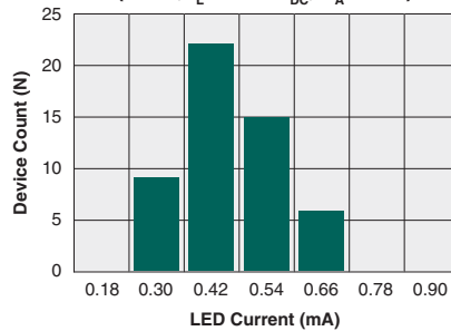
Typical I F for Switch Dropout (N=50, I L =120mA DC , T A =25°C)
