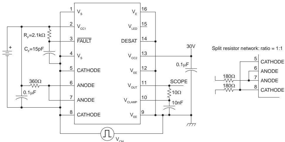
Figure 36. Driver CMR Test Circuit LED1 On
