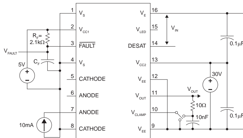
Figure 33. CMR Test Circuit LED2 Off
