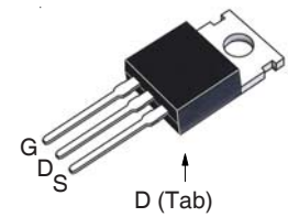
TO-220 (IXFP)
