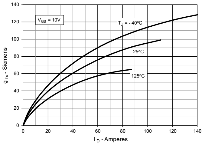
Fig. 9. Transconductance
