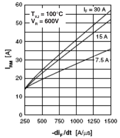
Fig. 23. Typ. peak reverse current I_{RM} versus -di_F/dt
