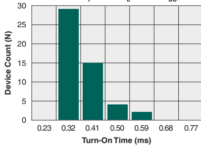
Form-A Typical Turn-On Time (N=50, I F =5mA, I L =170mA DC )
