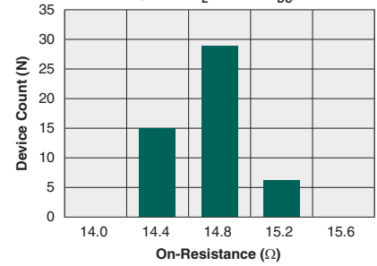
Form-A Typical On-Resistance Distribution (N=50, I L =170mA DC )
