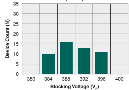
Form-A Typical Blocking Voltage Distribution (N=50)
