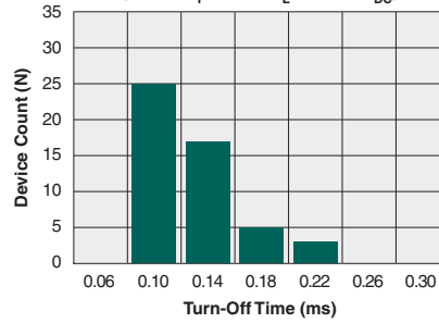
Form-A Typical Turn-Off Time (N=50, I F =5mA, I L =170mA DC )
