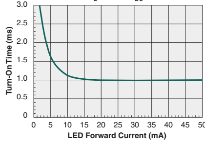
Typical Turn-On Time vs. LED Forward Current (I L =130mA DC )
