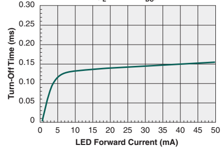
Typical Turn-Off Time vs. LED Forward Current (I L =130mA DC )
