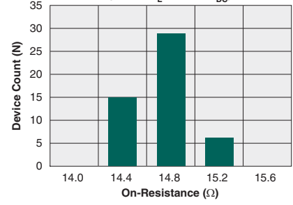
Typical On-Resistance Distribution (N=50, I_L=170mA_{DC} )
