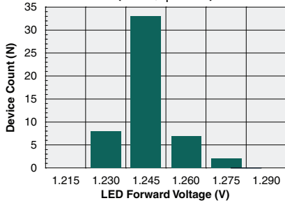
Typical LED Forward Voltage Drop (N=50, I_F=5mA )
